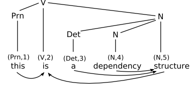
Figure 1: Representation of a dependency structure with a tree. The arrows below the words correspond to its associated dependency graph.
