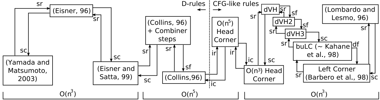
Figure 3: Formal relations between several well-known dependency parsers. Arrows going upwards correspond to generalisation relations, while those going downwards correspond to filtering. The specific subtype of relation is shown in each arrow’s label, following the notation in Section 4.
