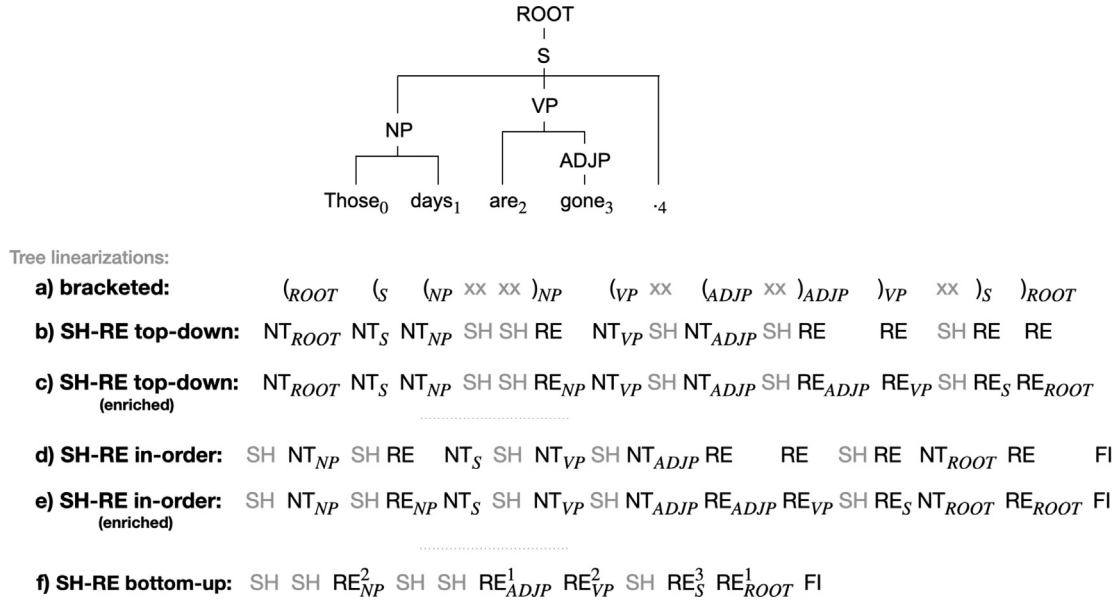
Fig. 2. Bracketed and shift-reduce (SH-RE) tree linearizations for encoding the continuous constituent tree in Fig. 1(a). SH = SHIFT, NT X = NON-TERMINAL-X, RE = REDUCE, RE X = REDUCE-X, RE X k = REDUCE#K-X and FI = FINISH.
