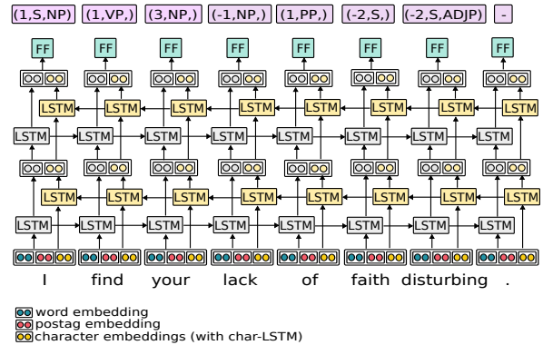
Figure 2: The baseline architecture used in this work.
