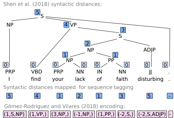
Figure 5: A constituent with syntactic distances attached to each non-terminal symbol, according to Shen et al. (2018). Distances can be used for sequence tagging, providing additional information to our base encoding (Gómez-Rodríguez and Vilares, 2018)
